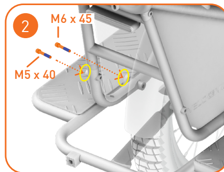
LOADY Trailer Adapter Platte
